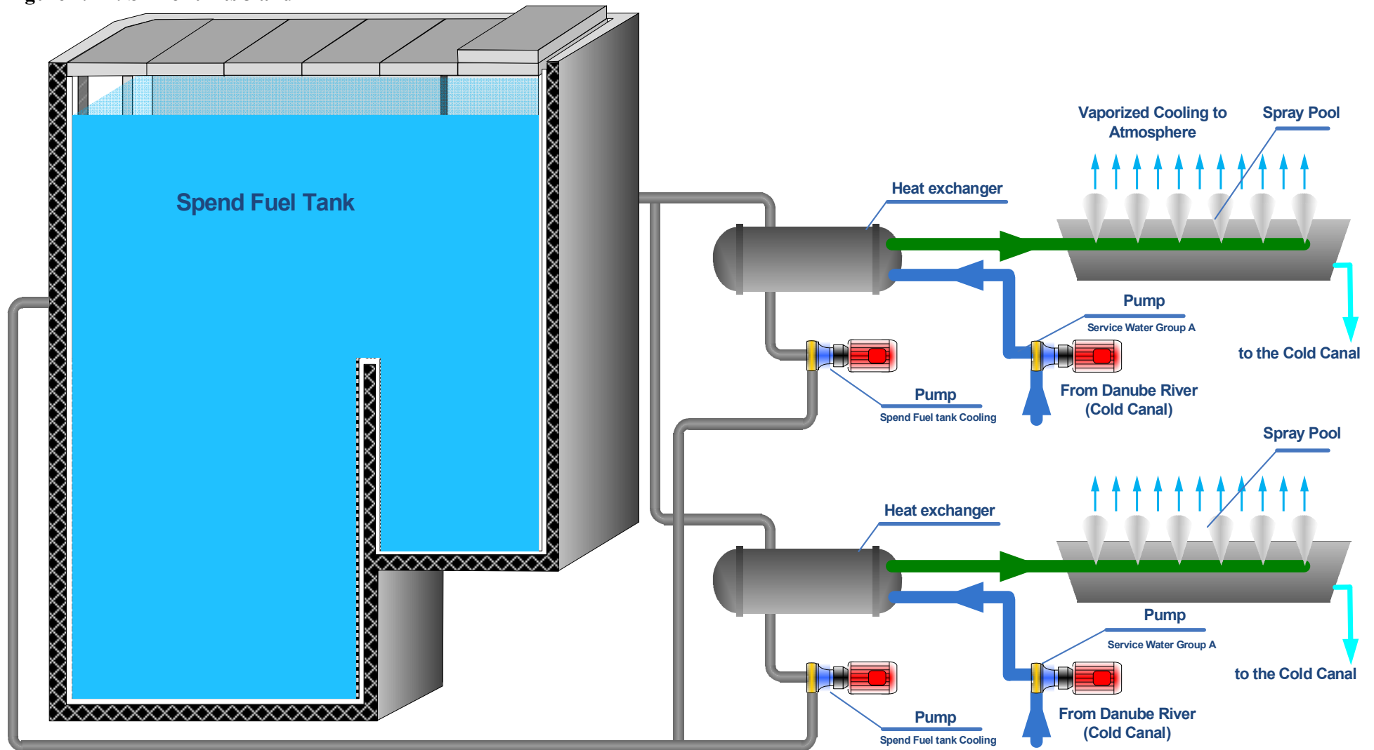
Figure 1.2-1: SFP of units 3 and 4
