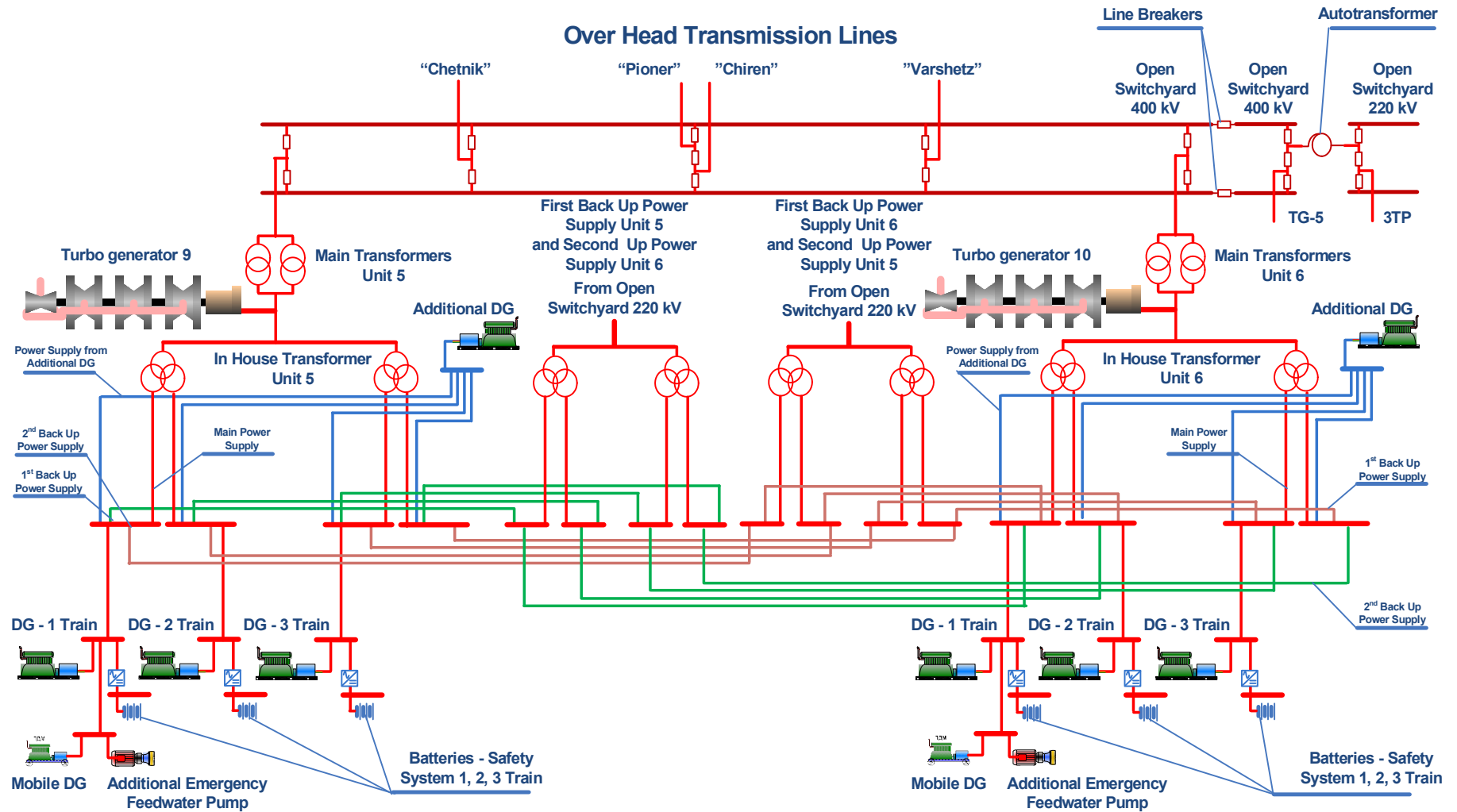
Figure 1.6-2: OSY 400 kV, Units 5 and 6
