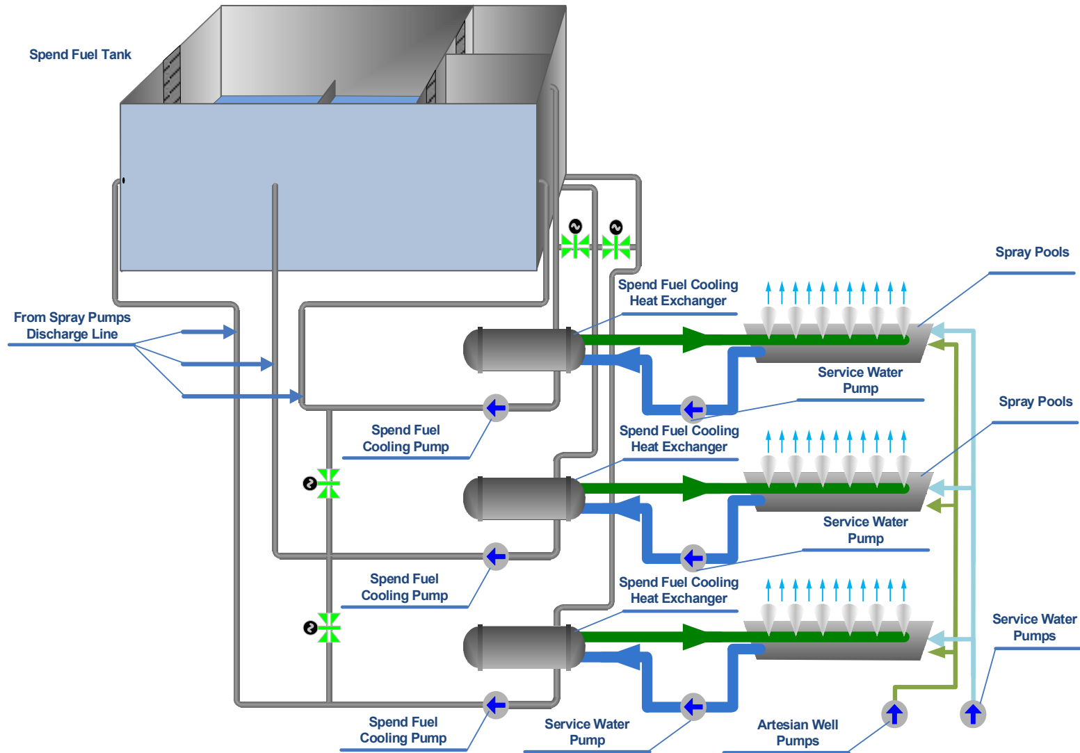
Figure 1.3-3: SFP for Units 5 and 6
