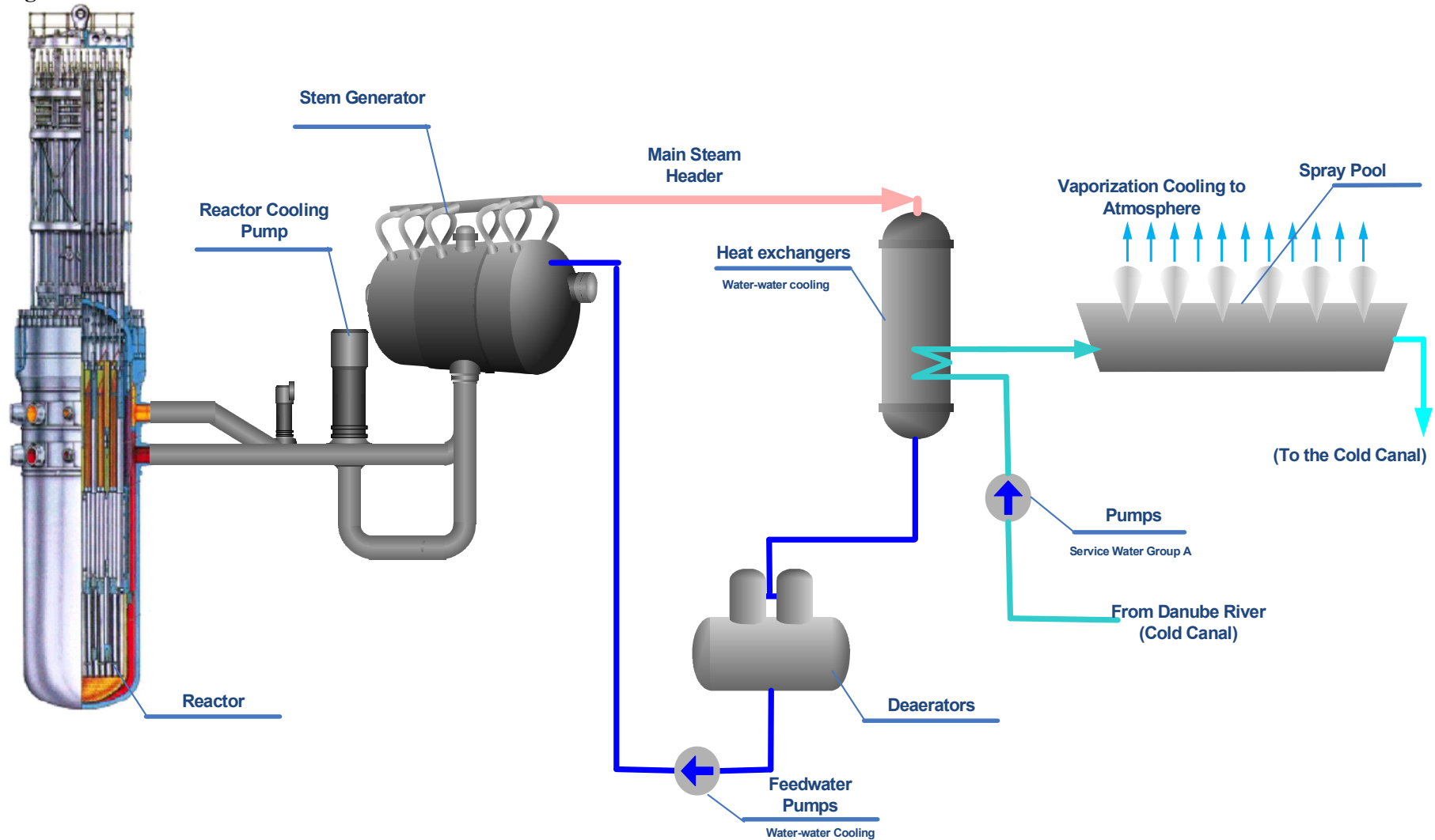
Figure 1.2-3: Ultimate heat sink
