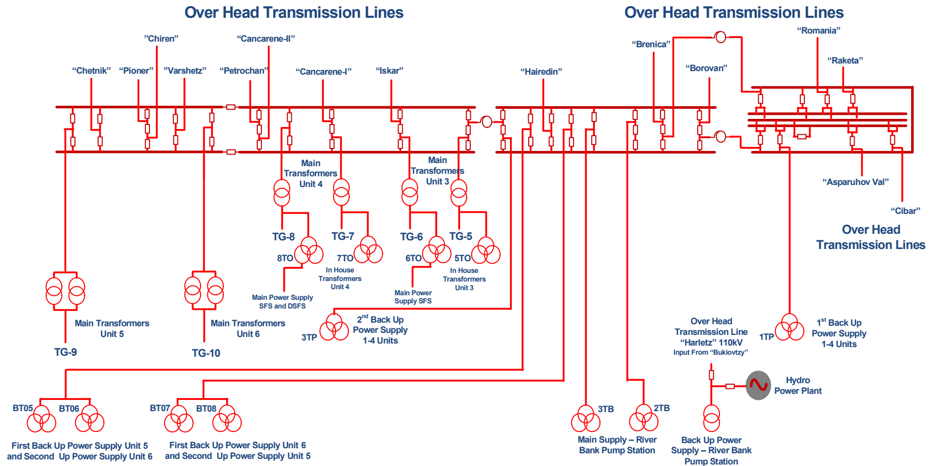
Figure 1.6-1: OSY diagram
