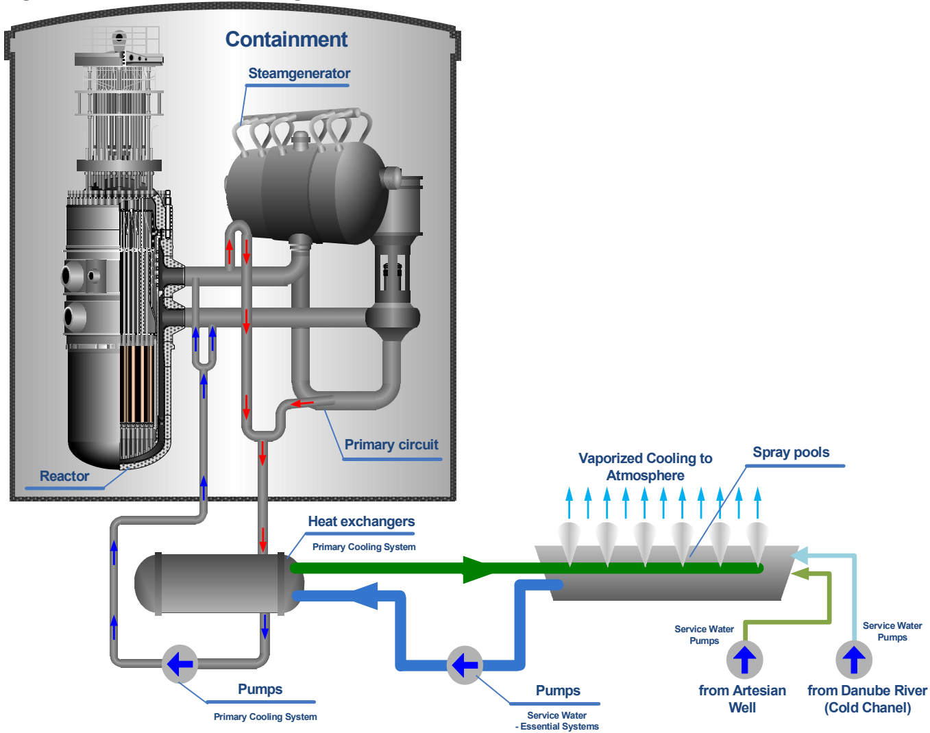
Figure 1.3-2: Water-water cooling
